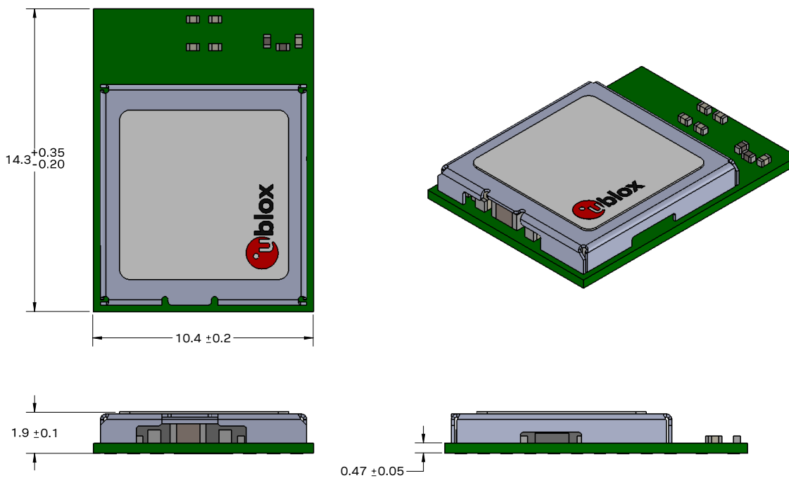
Figure 5: NORA-W306 mechanical specification
