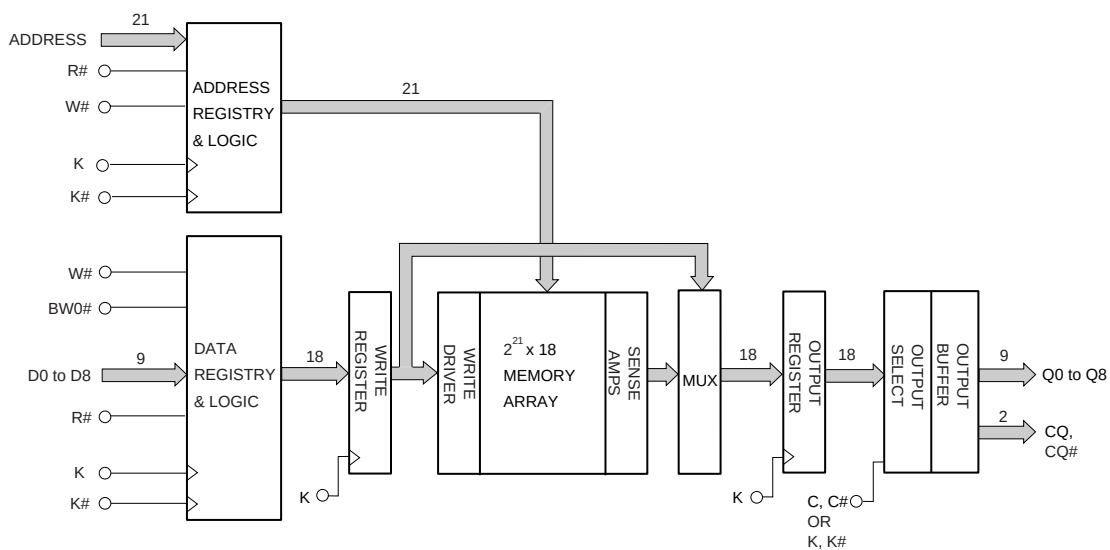
[μPD44325182B]
