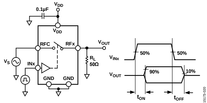
Figure 37. Switch Timing, t_{ON} and t_{OFF} (All RFx Terminals Connected to 50Ω Termination)
