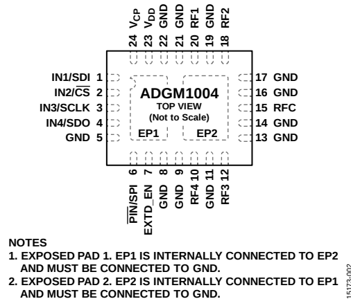
Figure 5. Pin Configuration
