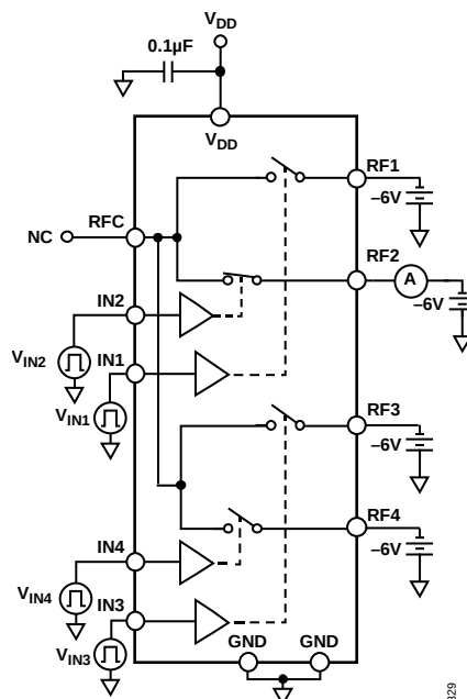
Figure 42. On Leakage
