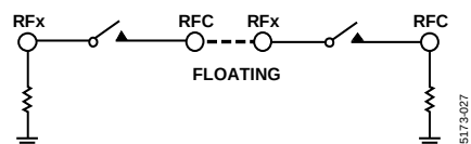
Figure 58. RFC Connected to RFx
