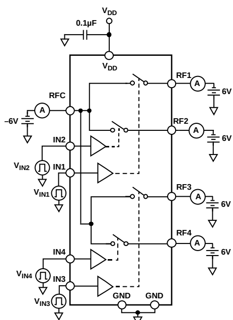
Figure 40. Off Leakage
