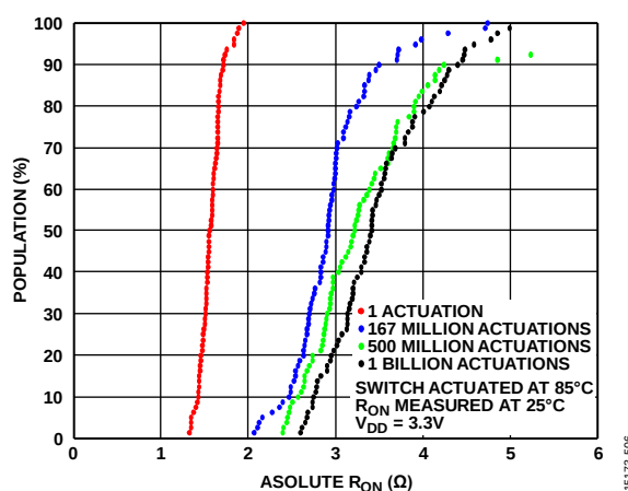
Figure 54. Population Percentage vs. Absolute R_{ON} , Switch Actuated at 85^\circ\text{C} and R_{ON} measured at 25^\circ\text{C}
