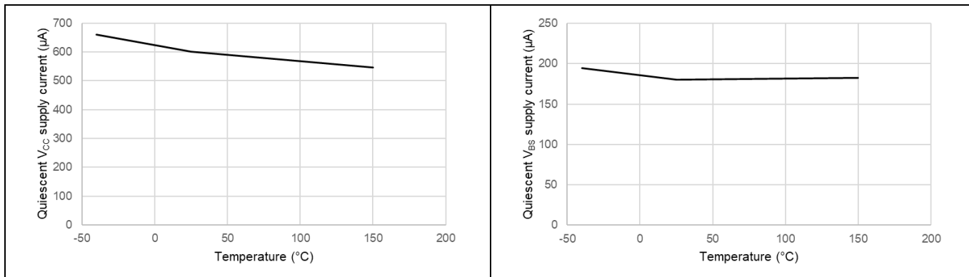
Figure 36 Quiescent V_{CC} and V_{BS} supply current
