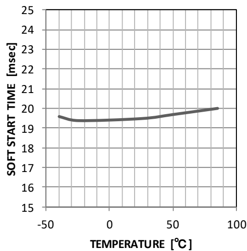
Fig.10 Soft Start Time - Temperature
