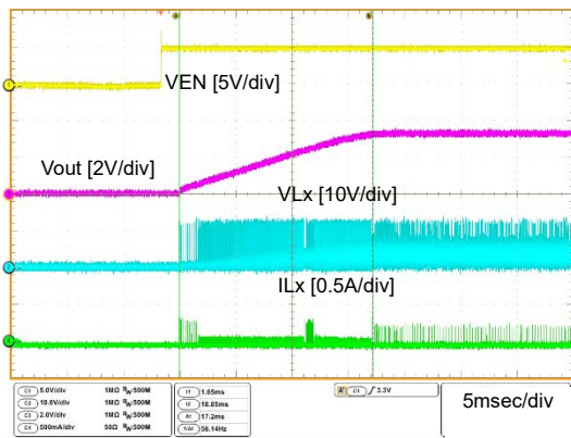
Fig.23 Start-up Characteristics
