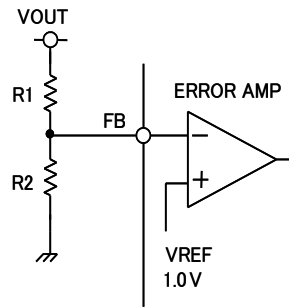
Fig.36 Output voltage setting
