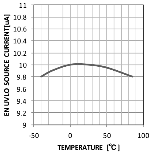
Fig.13 EN Source Current - Temperature
