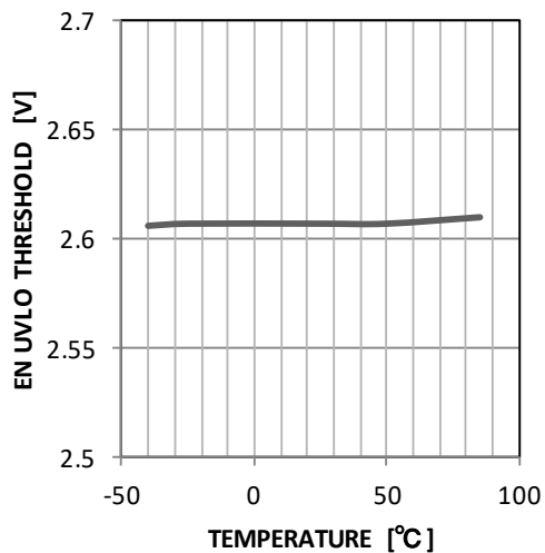
Fig.12 ENUVLO Threshold - Temperature
