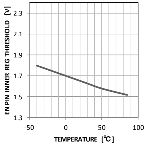
Fig.11 EN Pin Inner REG ON Threshold - Temperature
