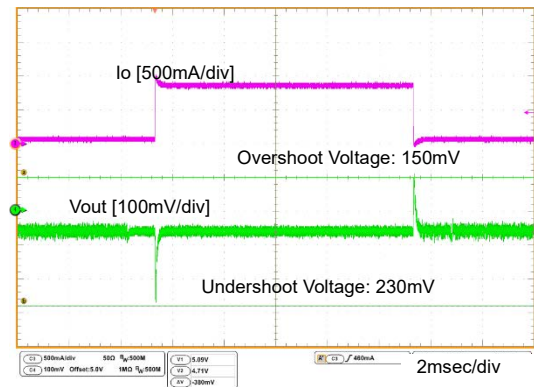
Fig.17 Load Response Iout:100mA \leftrightarrow 1A
