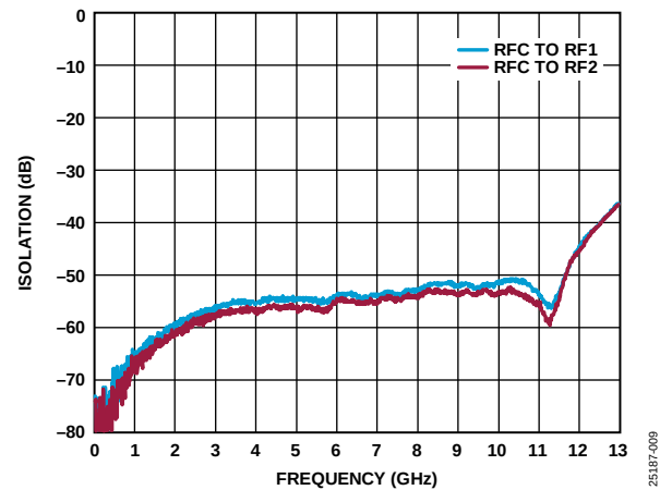
Figure 10. Isolation Between RFC and RFx vs. Frequency
