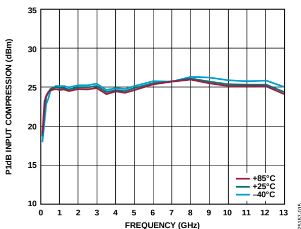
Figure 16. P1dB Input Compression Point vs. Frequency over Temperature, V_{CTRL} = -3\text{ V}
