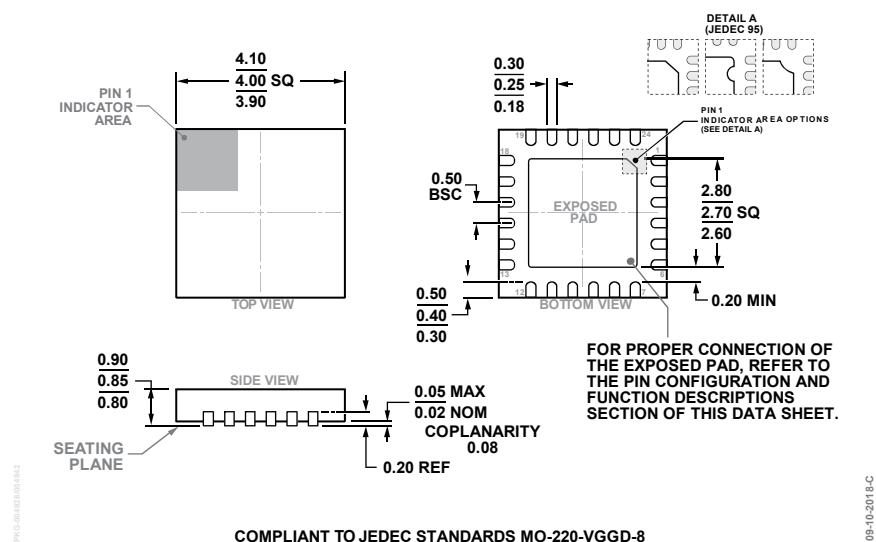
COMPLIANT TO JEDEC STANDARDS MO-220-VGGD-8 Figure 23. 24-Lead Lead Frame Chip Scale Package [LFCSP] 4 mm x 4 mm Body and 0.85 mm Package Height (CP-24-16) Dimensions shown in millimeters
