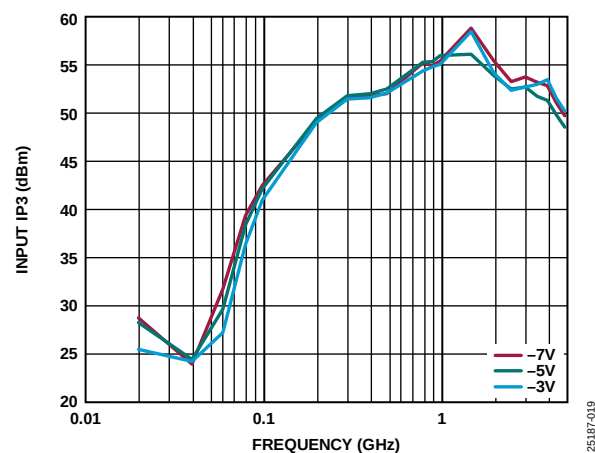
Figure 18. Input IP3 vs. Frequency over V_{CTRL} (Low Frequency Detail)
