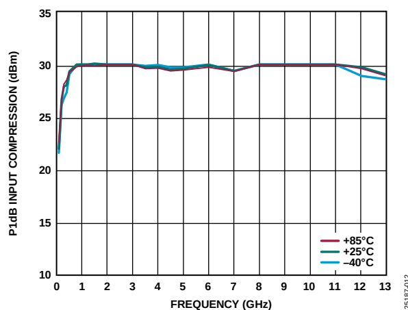
Figure 13. P1dB Input Compression Point vs. Frequency over Temperature, V_{CTRL} = -5\text{ V}
