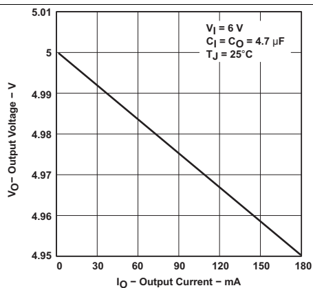
Figure 3. TPS76350-Q1 Output Voltage vs Output Current
