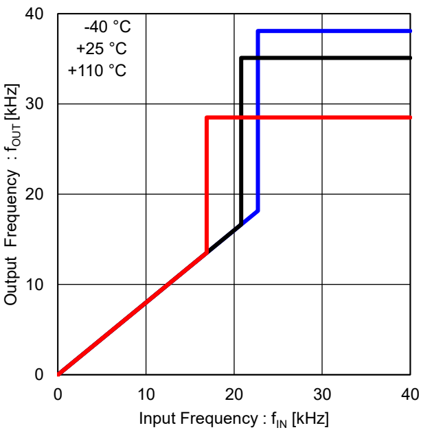
Figure 11. Output vs Input Frequency Characteristics
