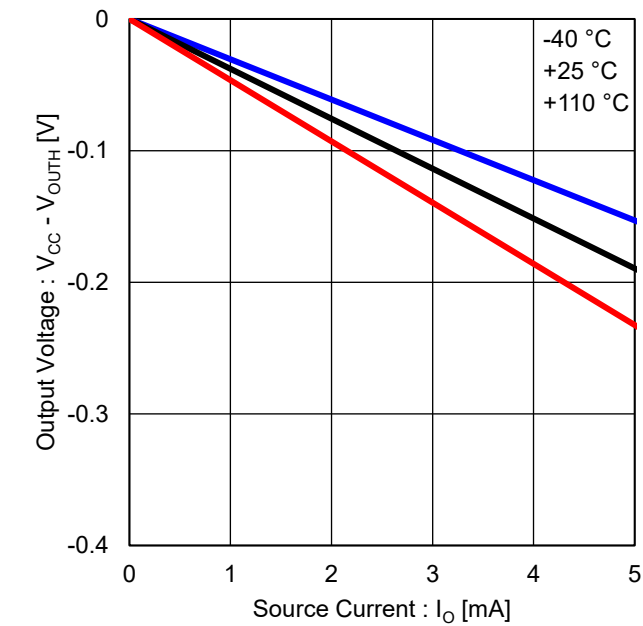
Figure 8. Output High Voltage
