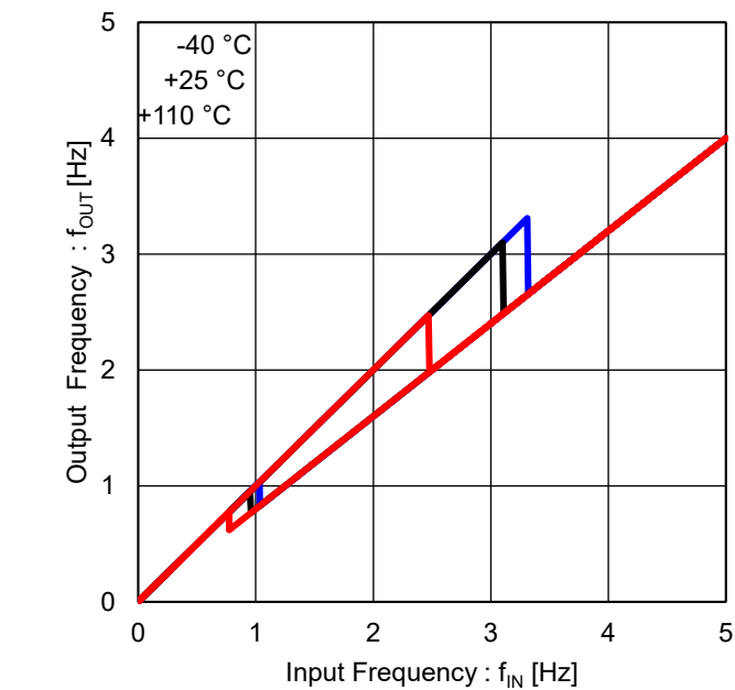
Figure 10. Output vs Input Frequency Characteristics (Low Frequency)
