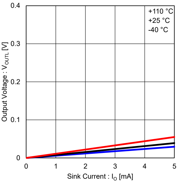
Figure 9. Output Low Voltage
