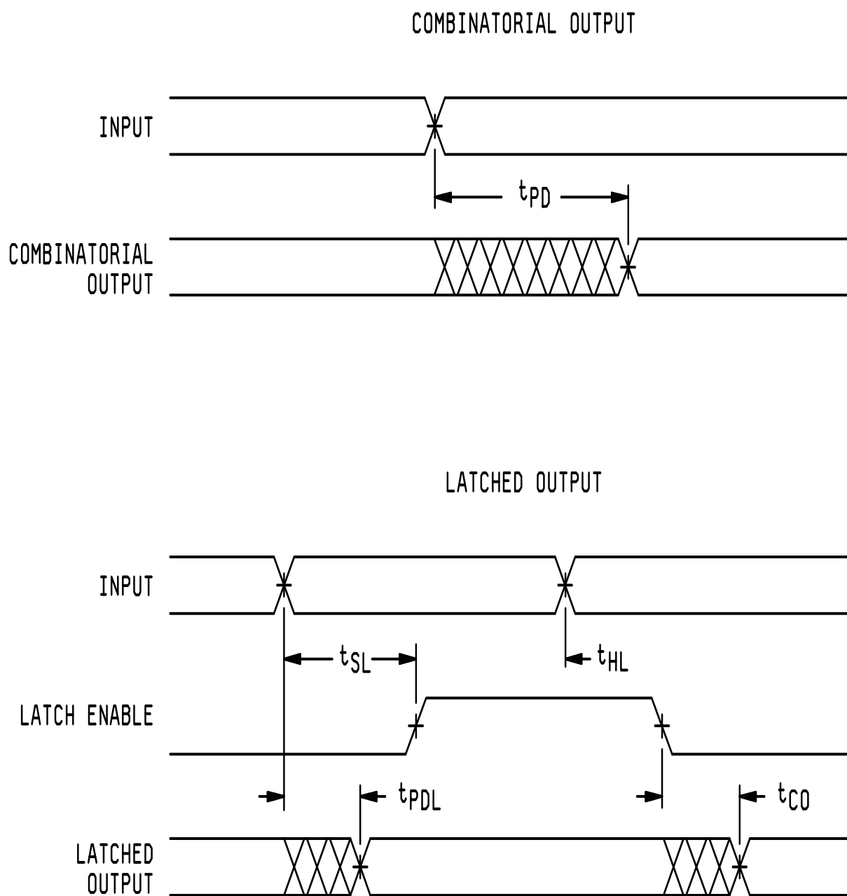
FIGURE 4. Switching waveforms.
