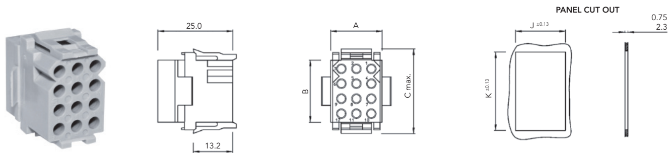
Panel Quick Mating mount receptacle (Delivered without contacts)
