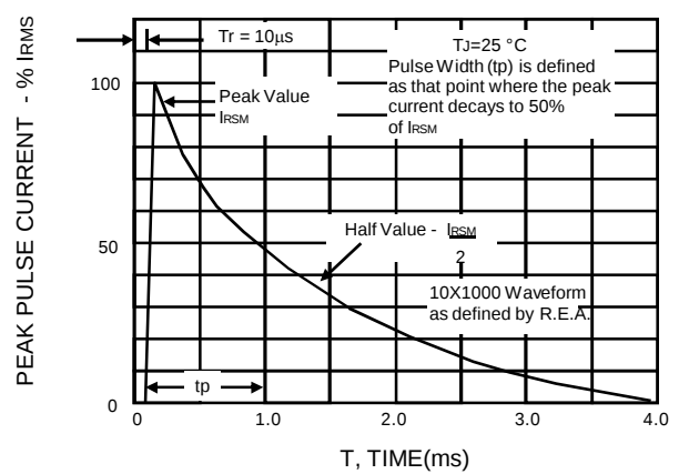
FIG.2 - PULSE WAVEFORM
