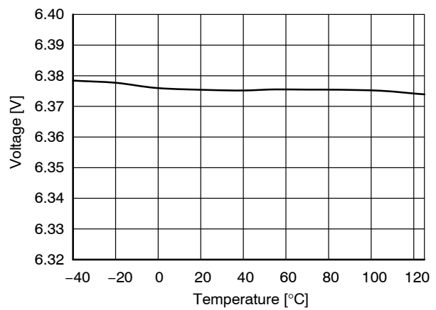
Figure 9. V_{Bon} vs. Temperature
