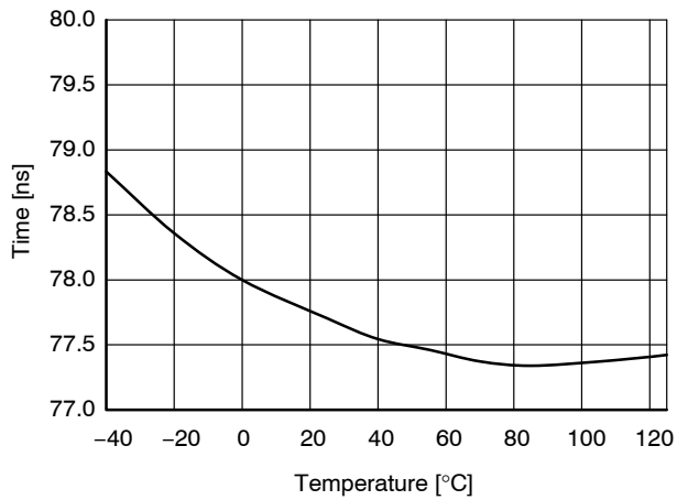
Figure 26. t_{DT} vs. Temperature (xB Version Only)
