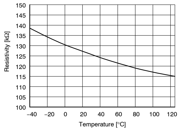
Figure 21. R_{EN} vs. Temperature
