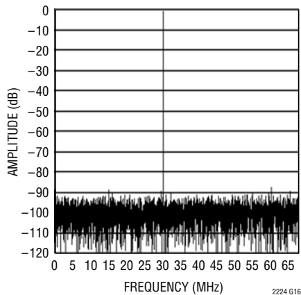
LTC2224: 8192 Point FFT, f_{IN} = 30\text{MHz} , -1\text{dB} , 1\text{V} Range
