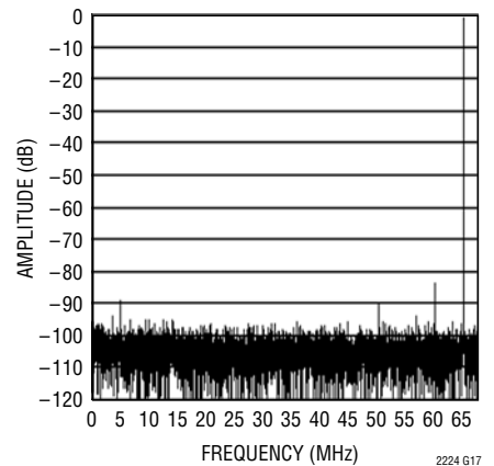
LTC2224: 8192 Point FFT, f_{IN} = 70\text{MHz} , -1\text{dB} , 2\text{V} Range
