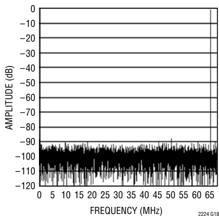
LTC2224: 8192 Point FFT, f_{IN} = 70\text{MHz} , -1\text{dB} , 1\text{V} Range
