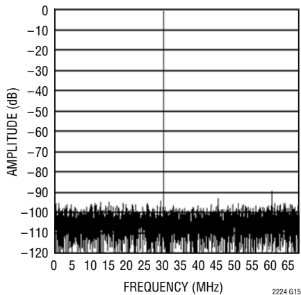
LTC2224: 8192 Point FFT, f_{IN} = 30\text{MHz} , -1\text{dB} , 2\text{V} Range
