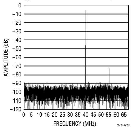
LTC2224: 8192 Point FFT, f_{IN} = 500\text{MHz} , -6\text{dB} , 1\text{V} Range
