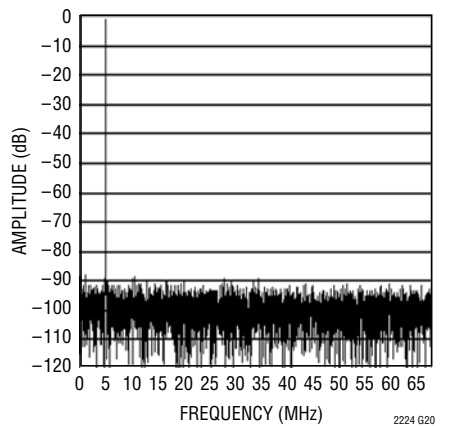
LTC2224: 8192 Point FFT, f_{IN} = 140\text{MHz} , -1\text{dB} , 1\text{V} Range
