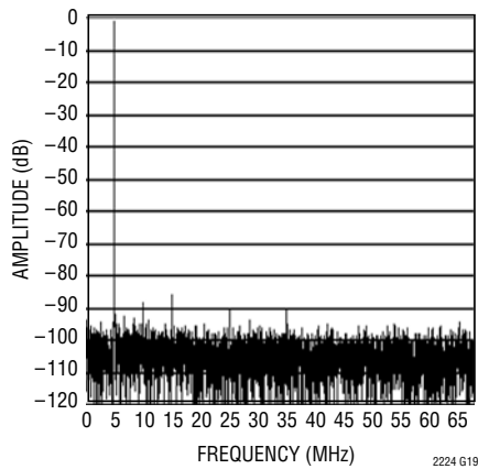
LTC2224: 8192 Point FFT, f_{IN} = 140\text{MHz} , -1\text{dB} , 2\text{V} Range
