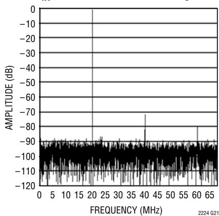
LTC2224: 8192 Point FFT, f_{IN} = 250\text{MHz} , -1\text{dB} , 2\text{V} Range
