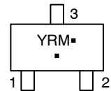
SC-59 CASE 318D
