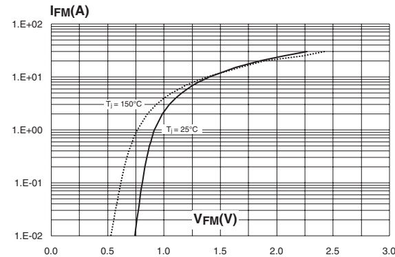
Fig. 9: Forward voltage drop versus forward current (typical values)
