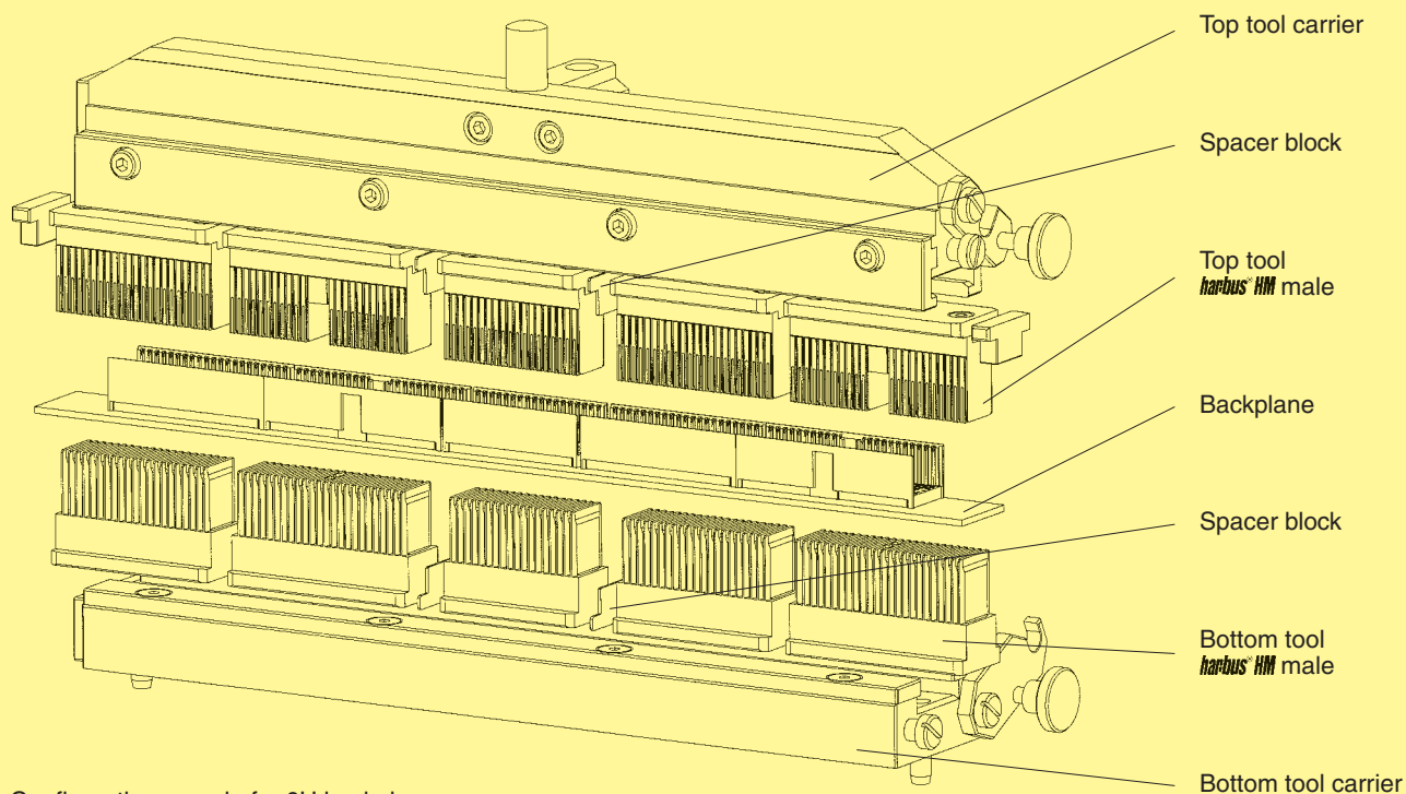
Configuration sample for 6U backplane
