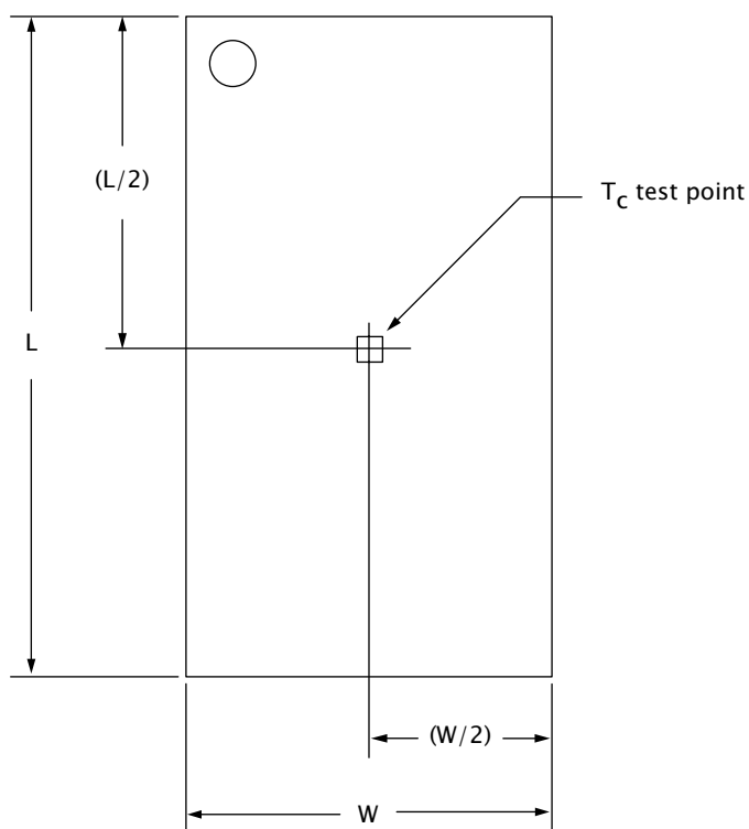
Figure 10: Thermal Measurement Point
