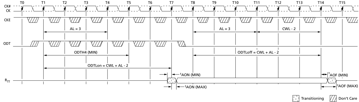
Figure 112: Synchronous ODT
