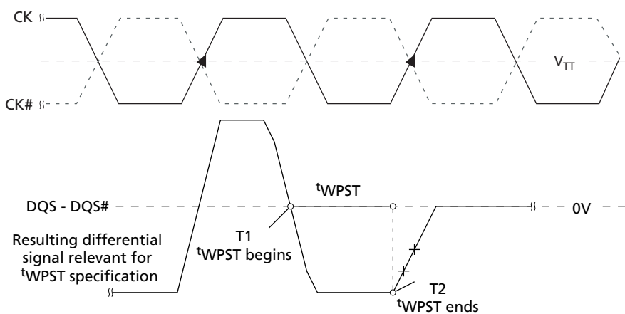
Figure 81: t_{WPST} Timing
