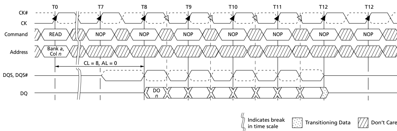
Figure 65: READ Latency
