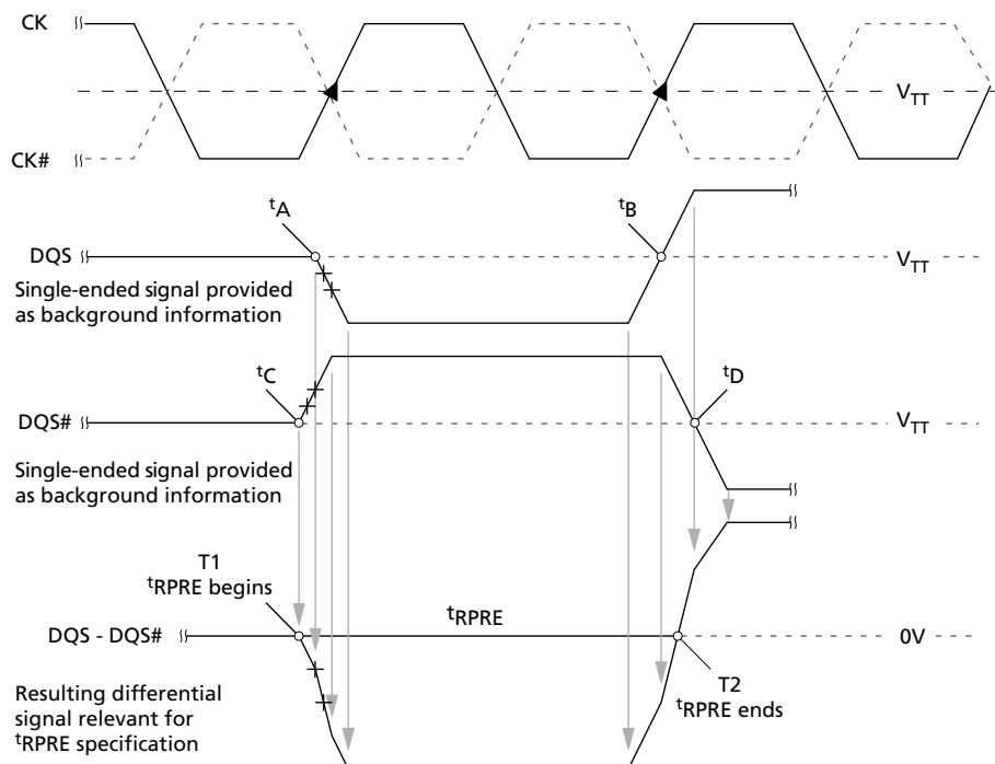
Figure 78: t_{RPRE} Timing
