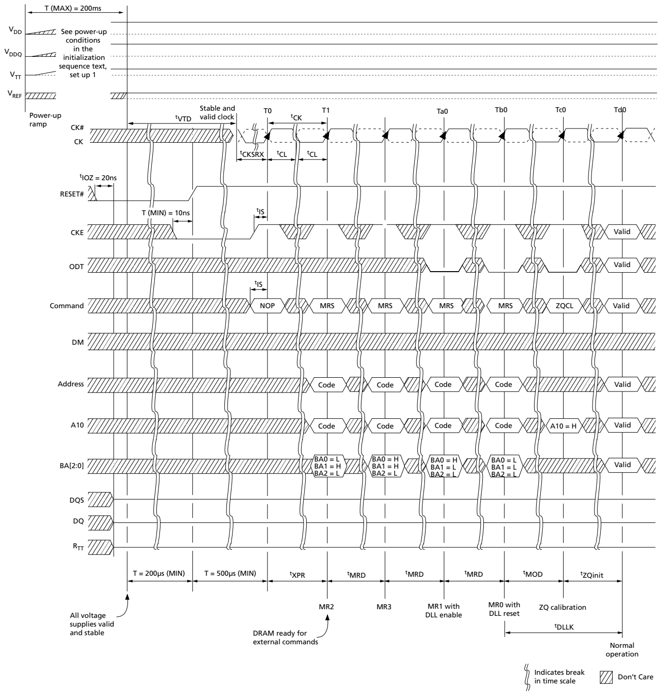
Figure 46: Initialization Sequence
