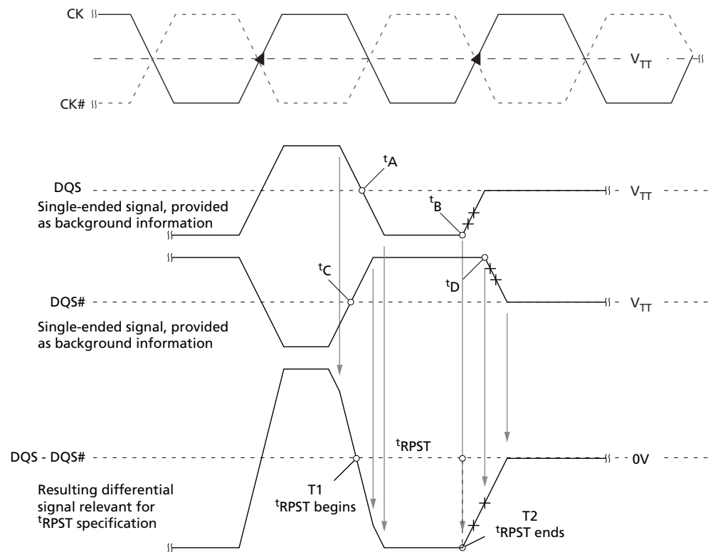
Figure 79: t_{RPST} Timing
