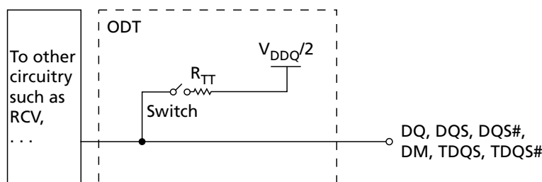
Figure 106: On-Die Termination
