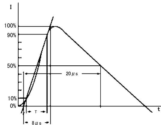
Fig. 8.2 Based on IEC61000-4-5 8/20 \mu\text{s} pulse.(Ed.2)
