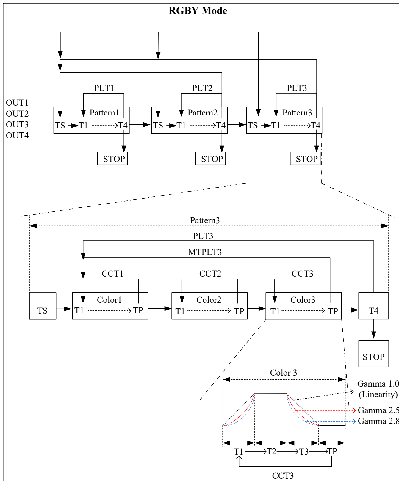
Figure 14 RGBY Mode
