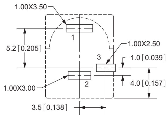
PCB LAYOUT
