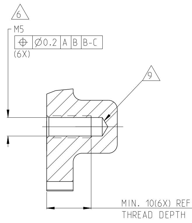
SECTION B-B
