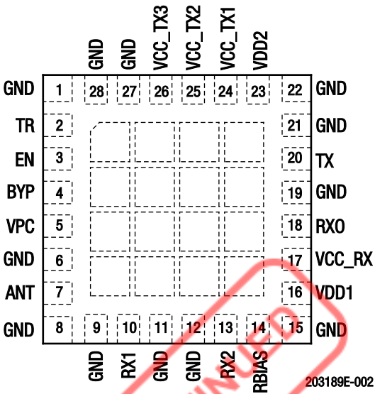
Figure 2. Figure 1. SKY65364-21 Pinout (Top View)
