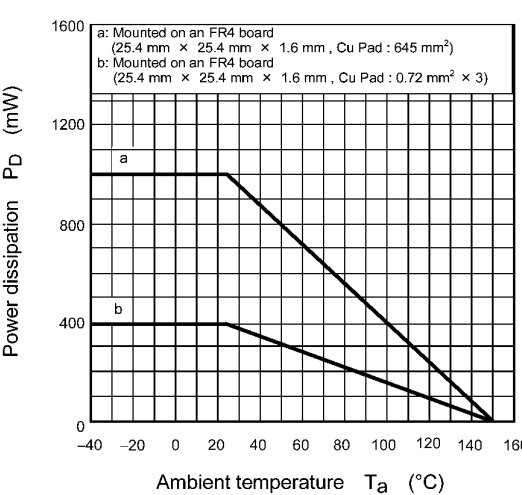
Fig. 8.12 P_D - T_a
