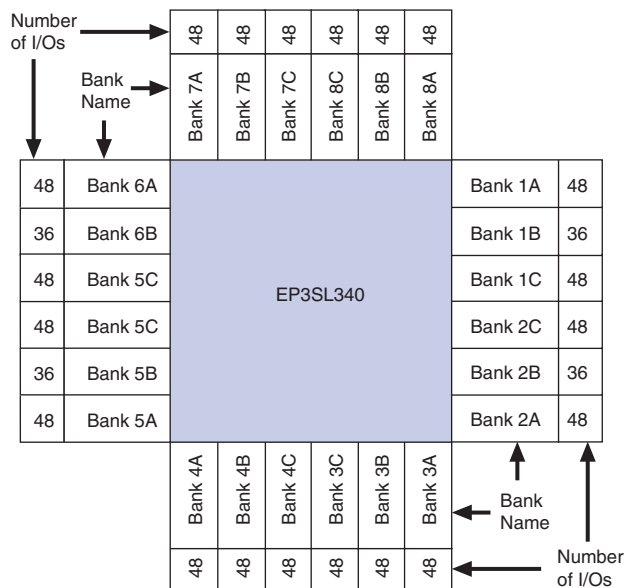
Figure 2-4. EP3SL340F1517 Device I/O Bank Diagram
