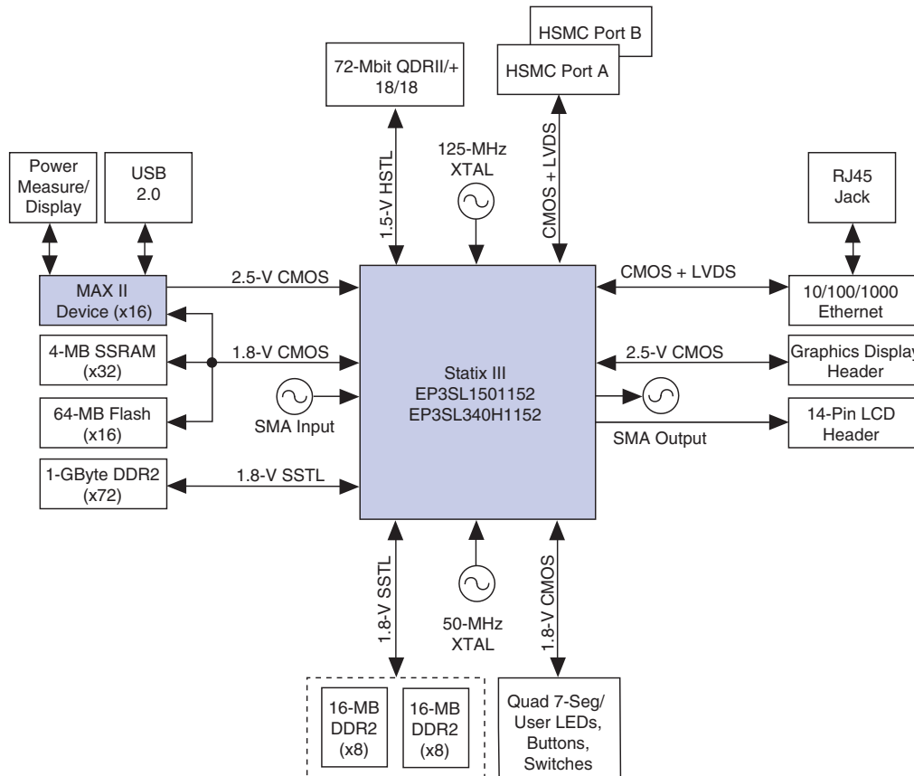
Figure 1–1. Stratix III Development Board Block Diagram
