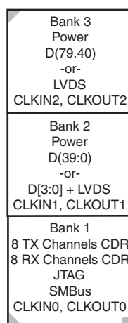
Figure 2-16. HSMC Signal and Bank Diagram
