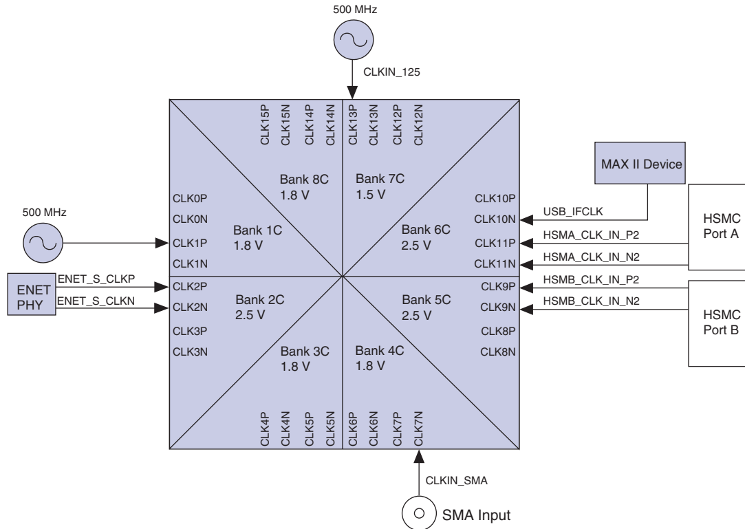
Figure 2-7. Stratix III FPGA Clock Inputs
