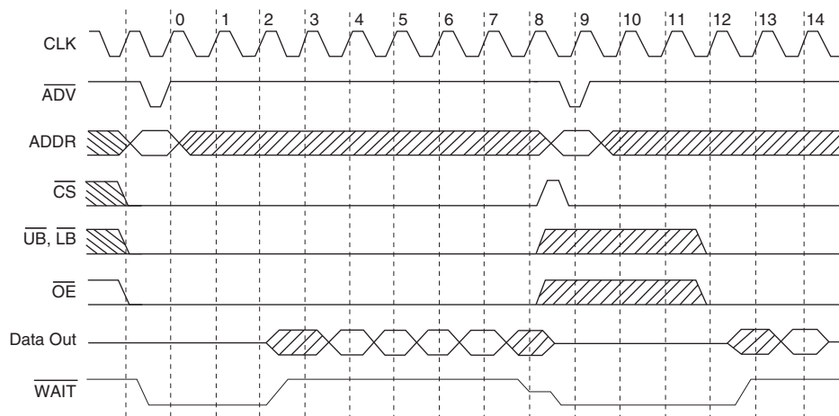
Figure 2-18. SRAM Read Timing Waveforms
