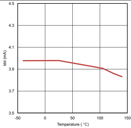
Figure 8. Operating Supply Current vs Temperature (Output Switching)
