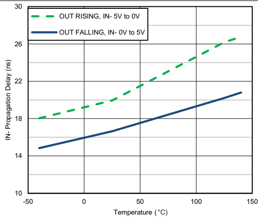
Figure 16. IN- Input-to-Output Propagation Delay vs Temperature
