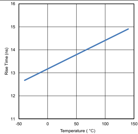
Figure 17. Rise Time vs Temperature
