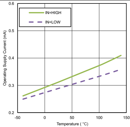
Figure 14. Operating Supply Current vs Temperature (Output in DC ON/OFF Condition)
