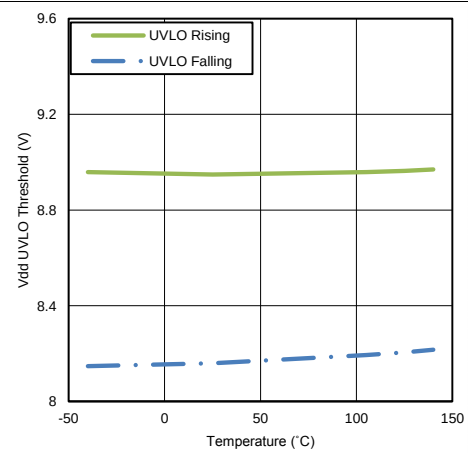
Figure 9. UVLO Threshold Voltage vs Temperature
