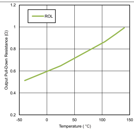
Figure 13. Output Pulldown Resistance vs Temperature
