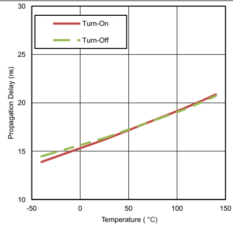
Figure 15. Input-to-Output Propagation Delay vs Temperature
