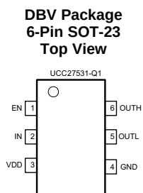
Pin Functions
