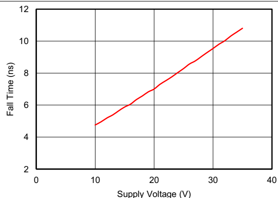
Figure 3. Fall Time vs Supply Voltage
