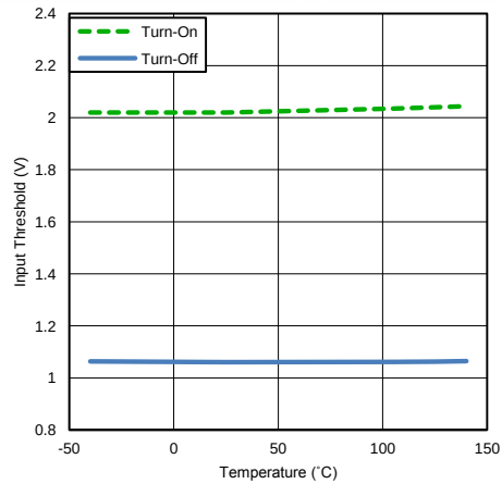
Figure 10. Input Threshold vs Temperature
