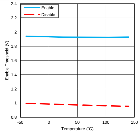
Figure 11. Enable Threshold vs Temperature
