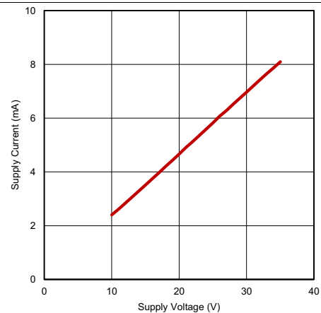
Figure 19. Operating Supply Current vs Supply Voltage (Output Switching)
