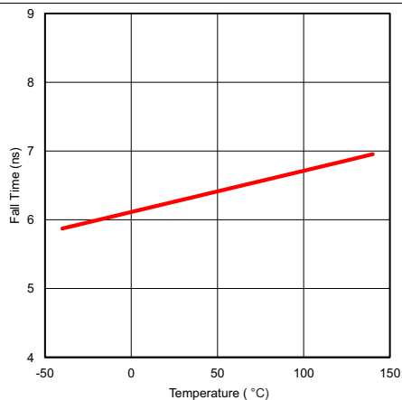
Figure 18. Fall Time vs Temperature
