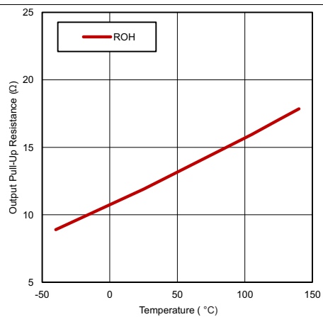
Figure 12. Output Pullup Resistance vs Temperature
