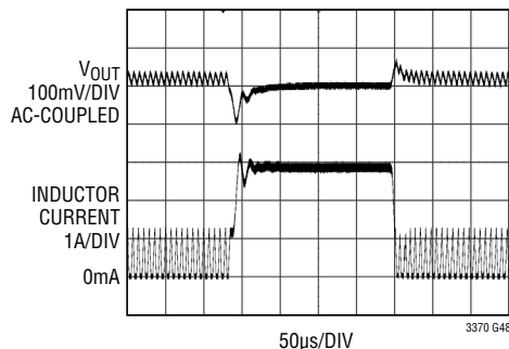
4A Buck Regulator, Transient Response (Burst Mode Operation)
