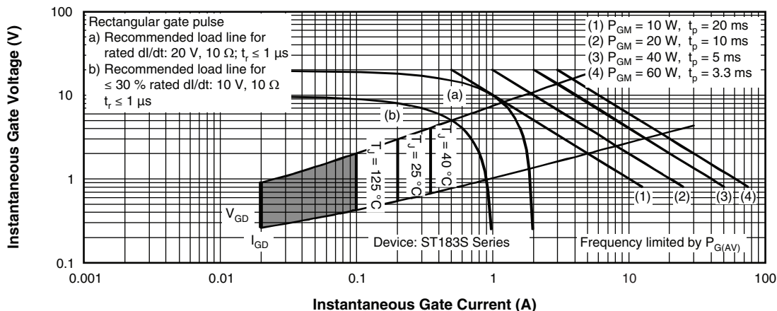
Fig. 15 - Gate Characteristics
