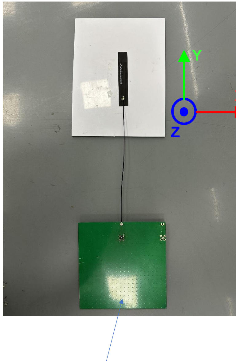
130 × 130 mm EVB
