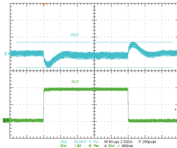
Figure 13: Load Step, CCM, V_{OUT} = 3.3V
