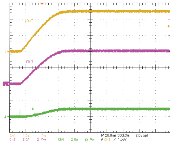
Figure 15: Start-Up, I_{OUT} = 4A
