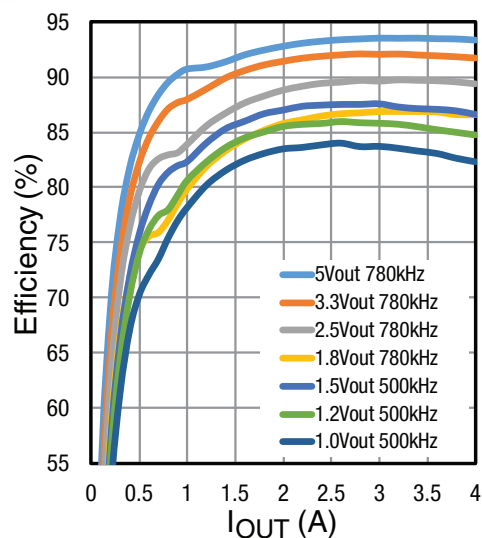
Figure 2: Efficiency 12VIN
