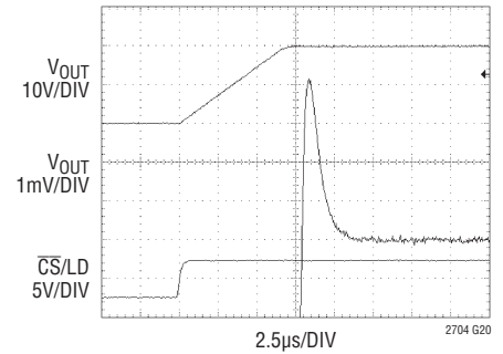
Settling \pm 10V
