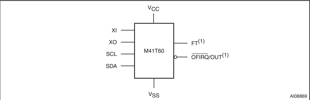
Figure 1. Logic diagram
