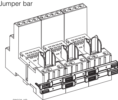
Jumper bar
