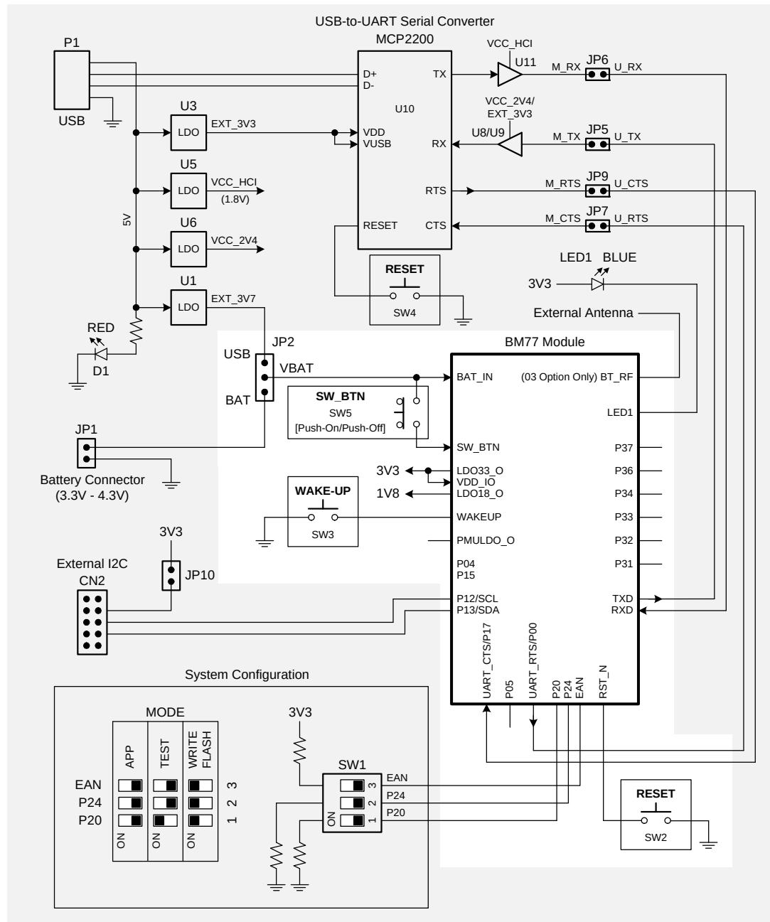
BM77 EVB BLOCK DIAGRAM
