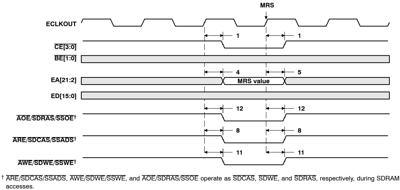
Figure 36. SDRAM MRS Command
