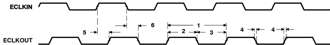
Figure 25. ECLKOUT Timings
