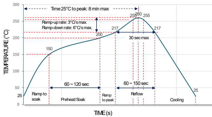
Reflow Profiles
