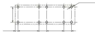
Recommended PC board pattern ( BOTTOM VIEW )
