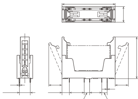
External dimensions
