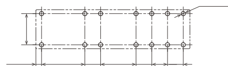
Recommended PC board pattern ( BOTTOM VIEW )
