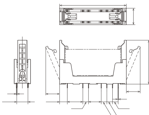
External dimensions
