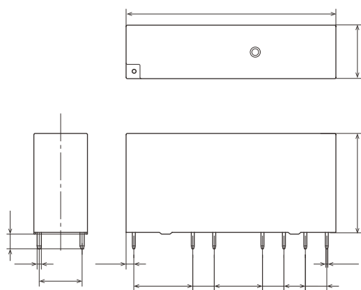
External dimensions
