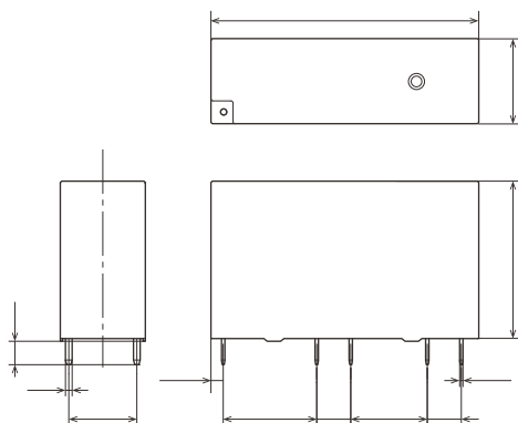
External dimensions
