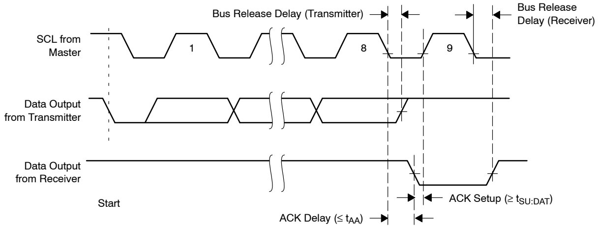
Figure 4. Acknowledge Timing
