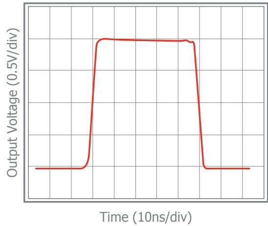
Large Signal Pulse Response at V S = 5V
