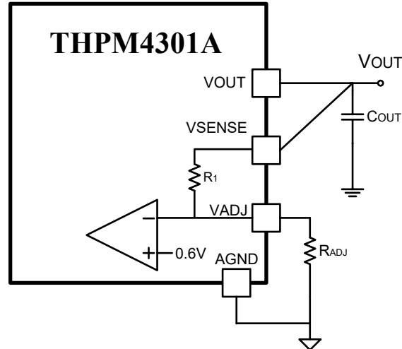
Fig. 15 Output Voltage Setting
