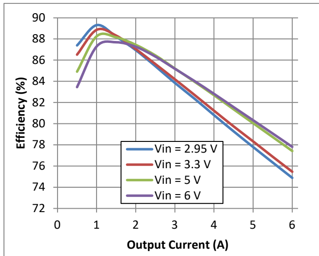
Fig. 13 Efficiency vs Output Current
