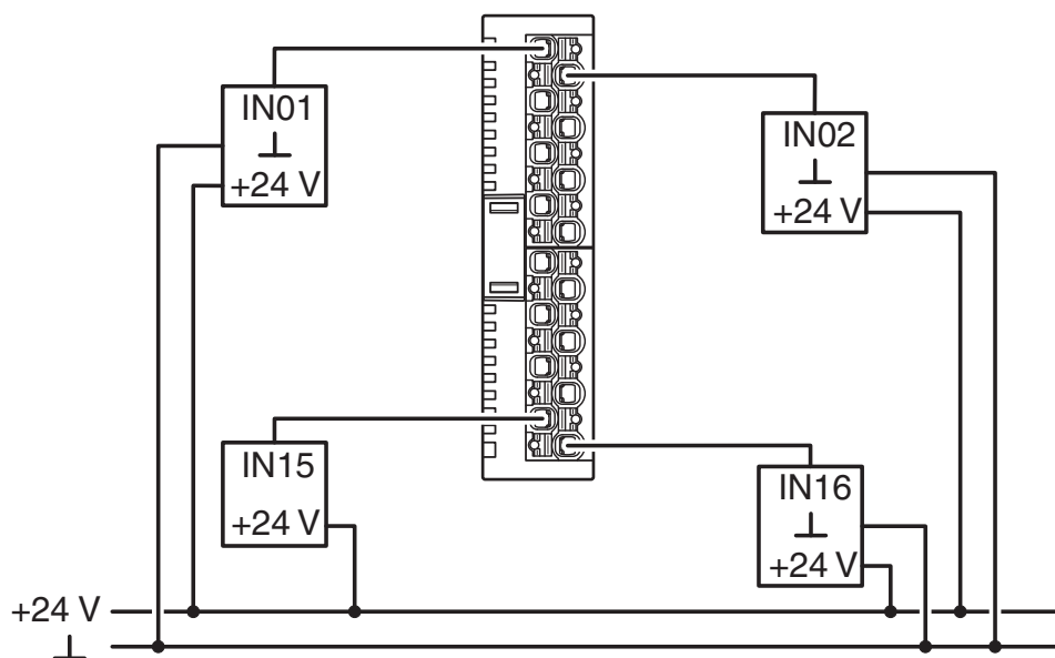
Connection in 1-conductor technology
