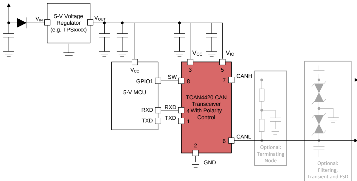
Figure 17. Typical CAN Bus Application Using TCAN4420 with 5 V \mu C
