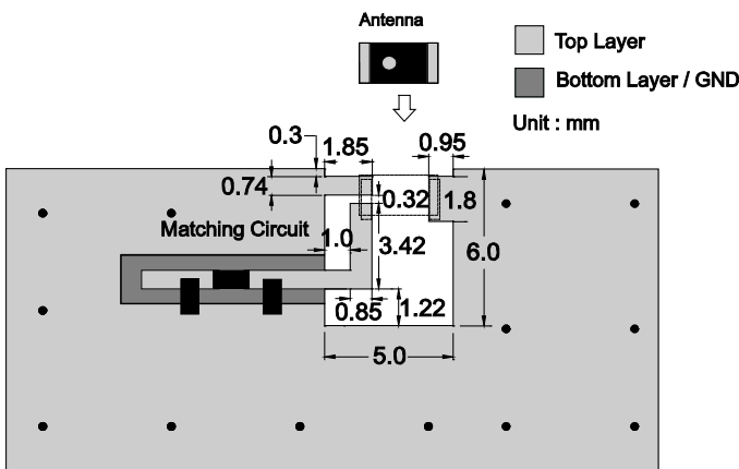
Fig. 2 Outlook and dimension of evaluation board
