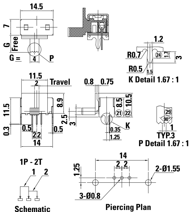
SK-12D26-G 6.5 NS 1P2T Non-Shorting 6.5mm Knob SK-12D26-G 6.5 NS GY 1P2T Non-Shorting 6.5mm Knob
