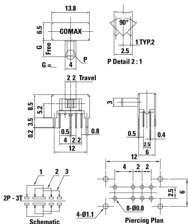
SK-23D24-G 4 2P3T 4mm Knob SK-23D24-G 7 2P3T 7mm Knob
