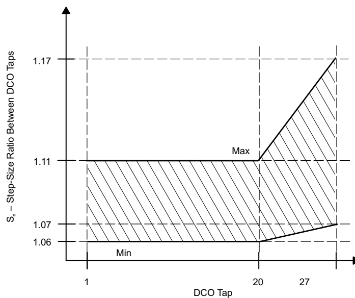
Figure 5-12. DCO Tap Step Size
