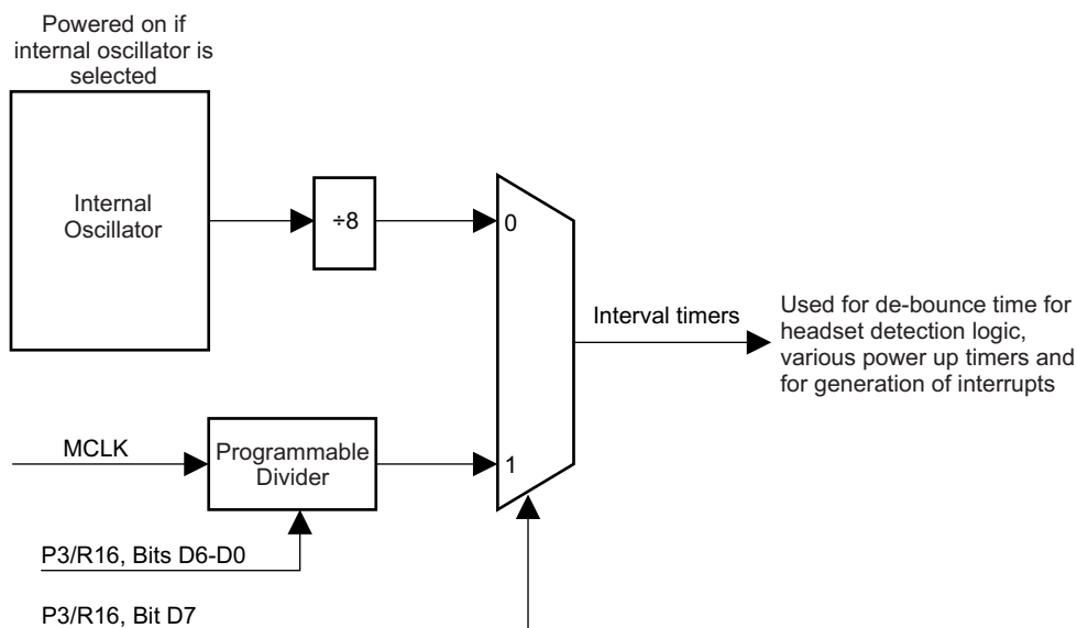
Figure 5-23. Interval Timer Clock Selection
