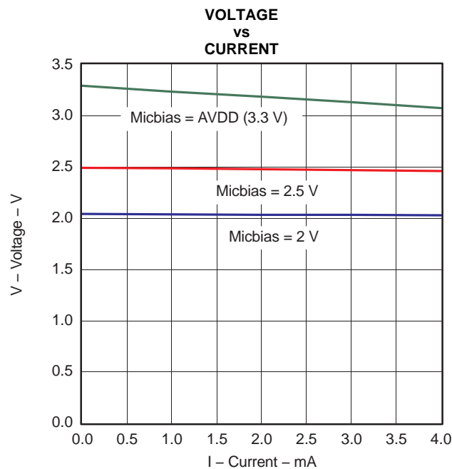
Figure 4-10. MICBIAS
