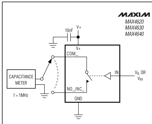
Figure 3. Channel Off/On-Capacitance
