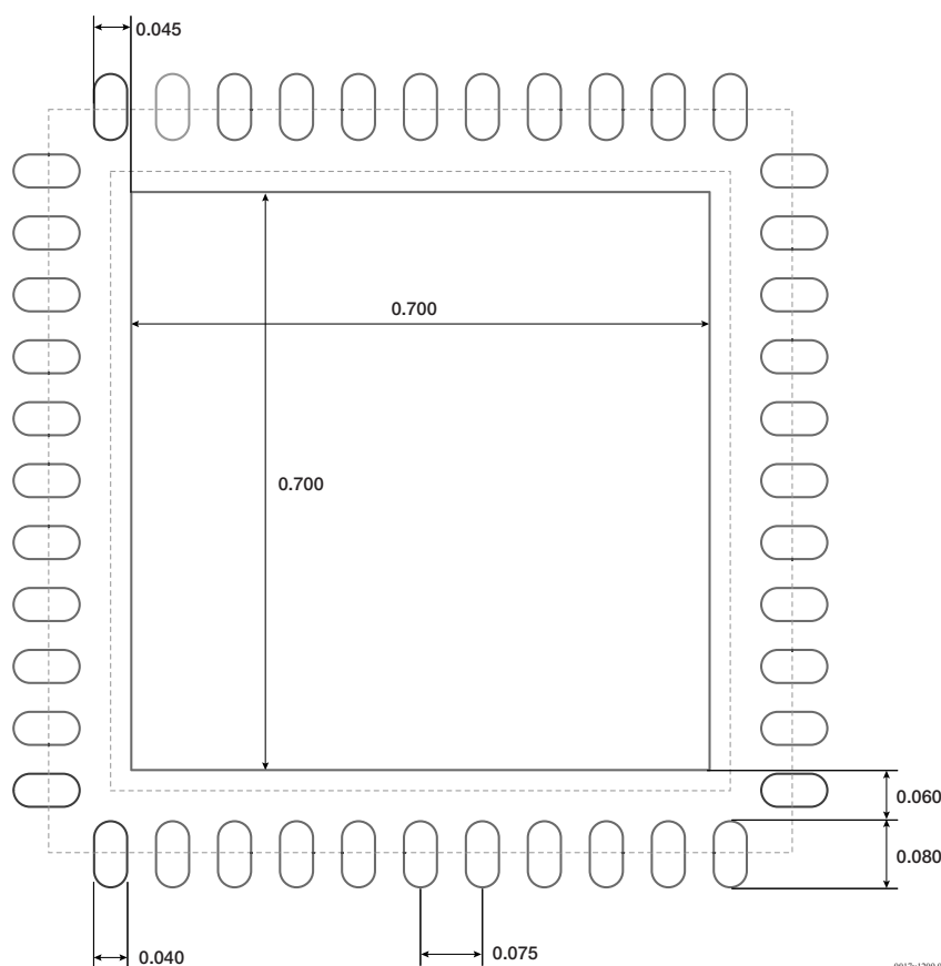
Figure 4-3 • Recommended PCB Layout
