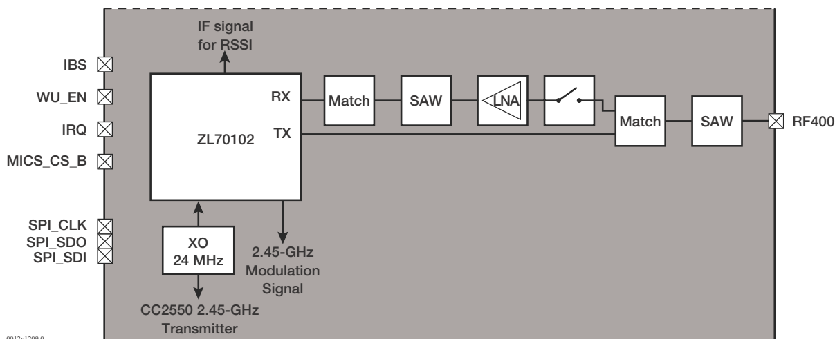
Figure 2-2 • MICS-Band RF Transceiver Circuit
