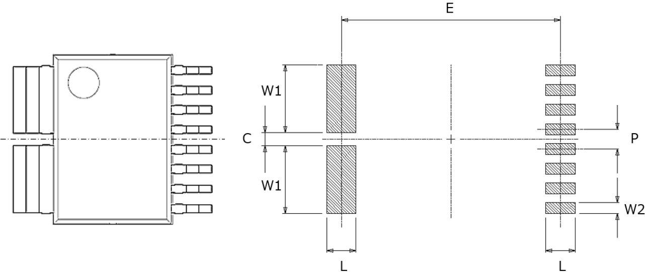
Figure 10. Recommended pad pattern
