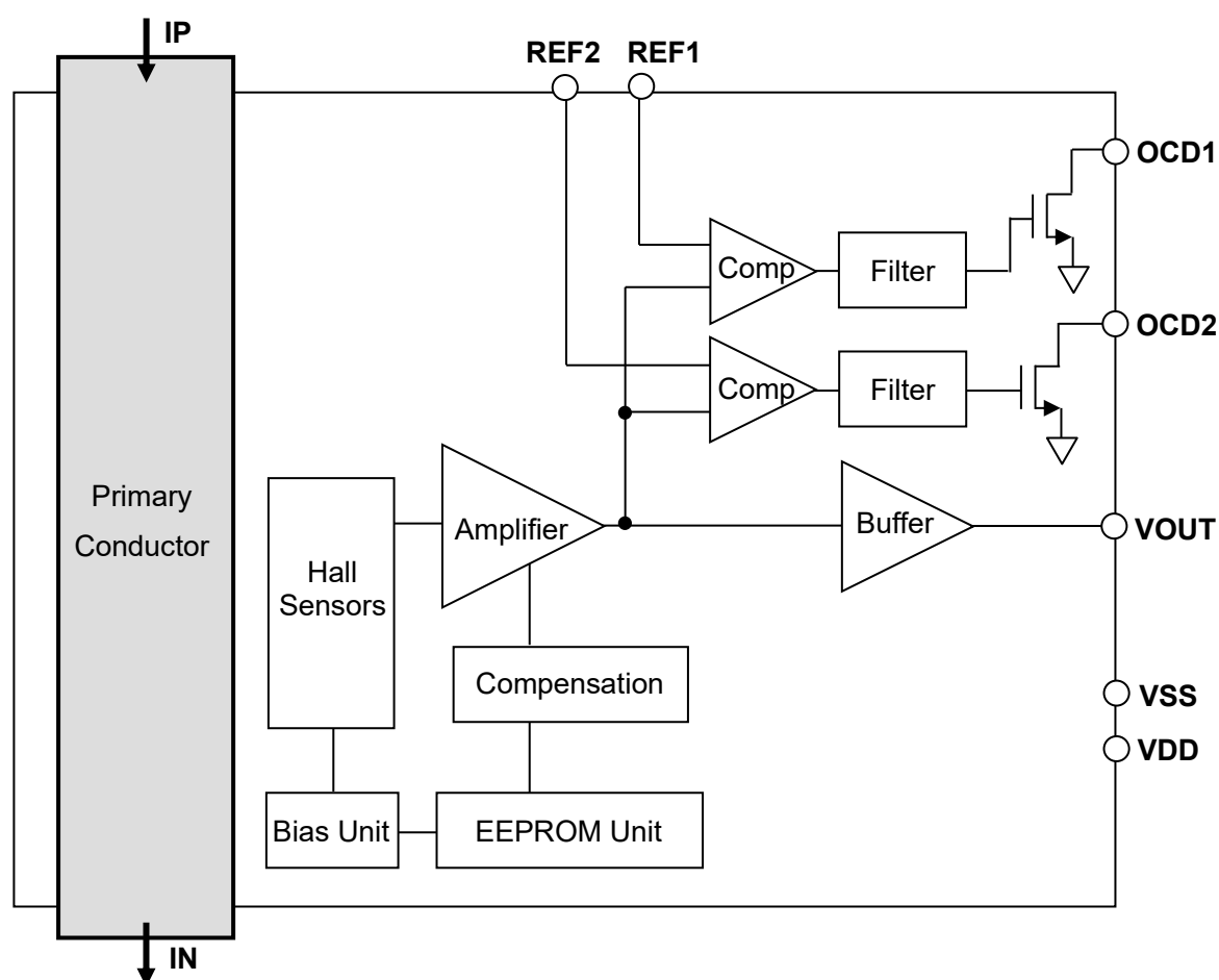
Figure 1. Block diagram of CZ-3A01
