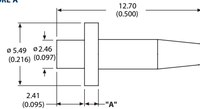
Pin P2-P3
