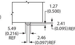
Pin P2-P3
