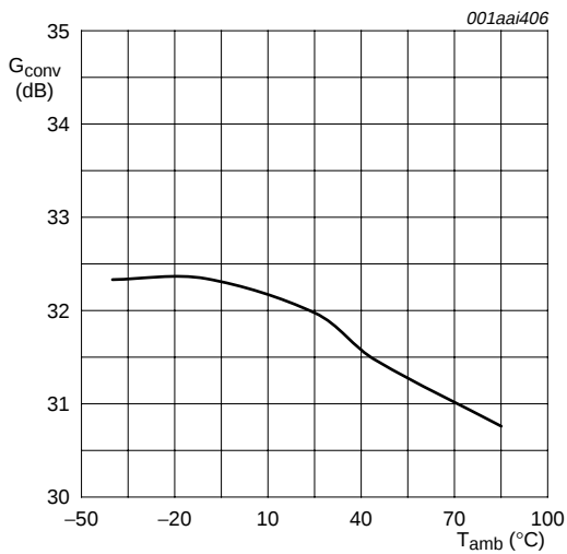
Fig 20. Conversion gain as function of temperature (high band); typical values
